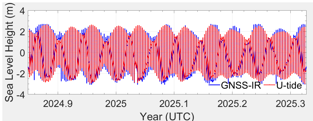
Figure 2: UTide Analysis
