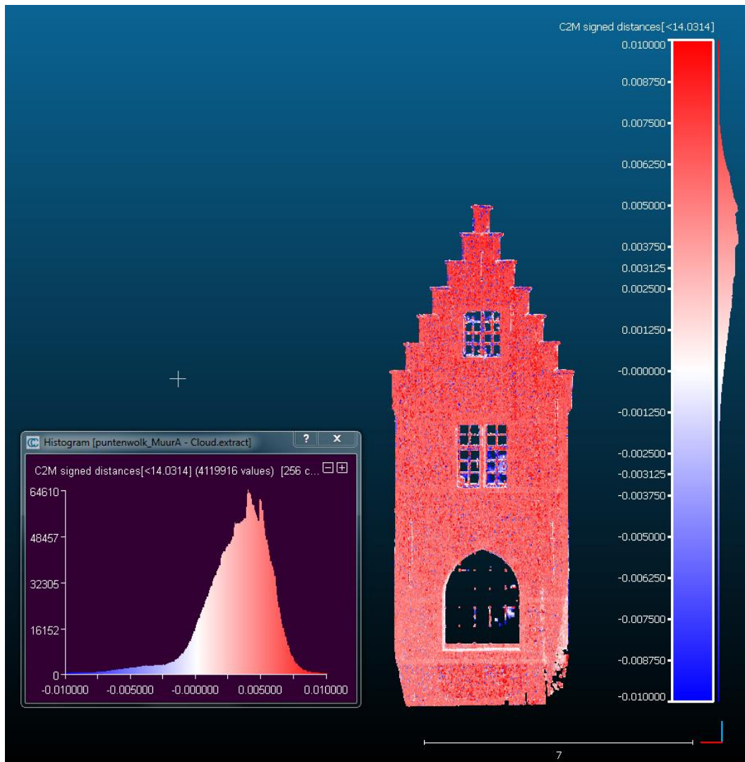
Figure 61: Difference model of the laser scan point cloud between 2 groups using Cloud Compare
